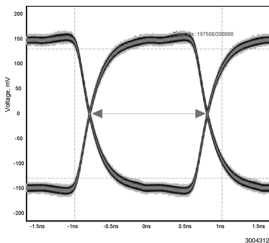
LVDS RxCLKOUT Output (3.125 Gbps, 20m CAT-6 SCTP, 0x001 DS32ELX0124 EQ setting, 0x10 DS32EL0421 De-Emphasis setting)
