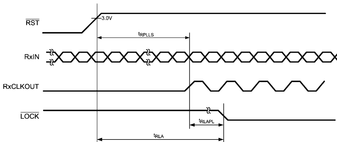
FIGURE 4. Reset to Lock Time
