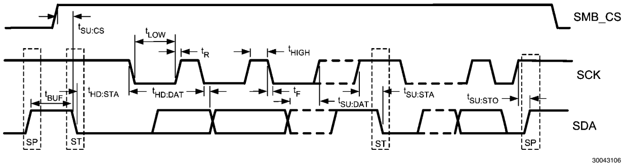
FIGURE 1. SMBus Timing Parameters
