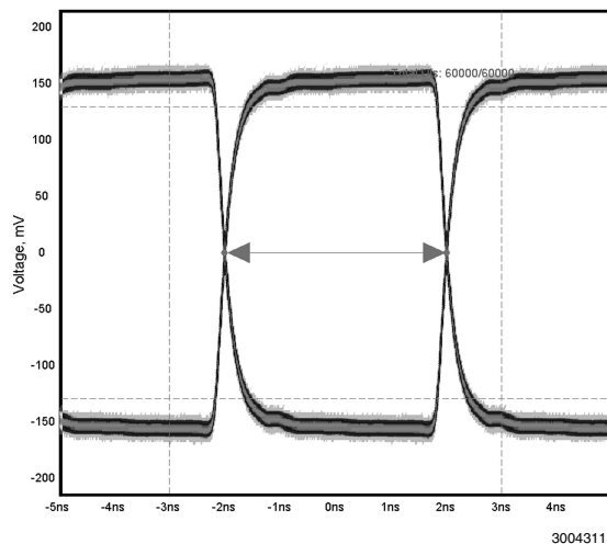
LVDS RxCLKOUT Output (1.25 Gbps, 40m CAT-5e, 0x000 DS32ELX0124 EQ setting, 0x10 DS32EL0421 De-Emphasis setting)
