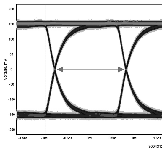
LVDS RxOUT0 Output (3.125 Gbps, 20m CAT-6 SCTP, 0x001 DS32ELX0124 EQ setting, 0x10 DS32EL0421 De-Emphasis setting)
