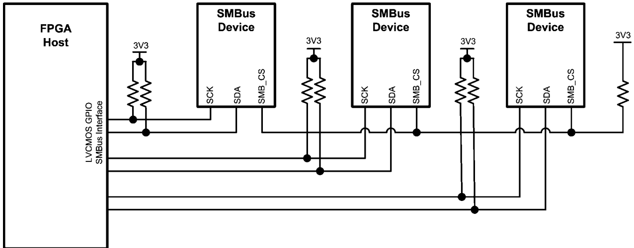
FIGURE 10. SMBus Configuration 3
