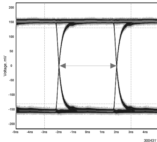
LVDS RxOUT0 Output (1.25 Gbps, 40m CAT-5e, 0x000 DS32ELX0124 EQ setting, 0x10 DS32EL0421 De-Emphasis setting)
