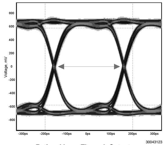
Retimed Loop Through Output (3.125 Gbps, 20m CAT-6 SFTP, 0x001 DS32ELX0124 EQ setting, 0x10 DS32EL0421 De-Emphasis setting)
