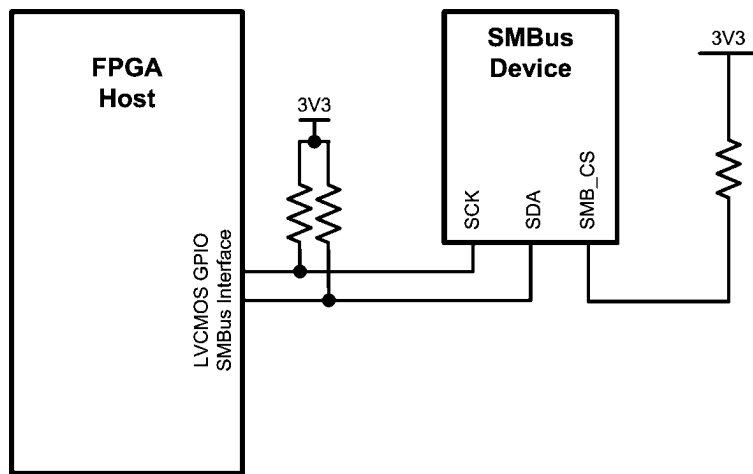
FIGURE 8. SMBus Configuration 1
